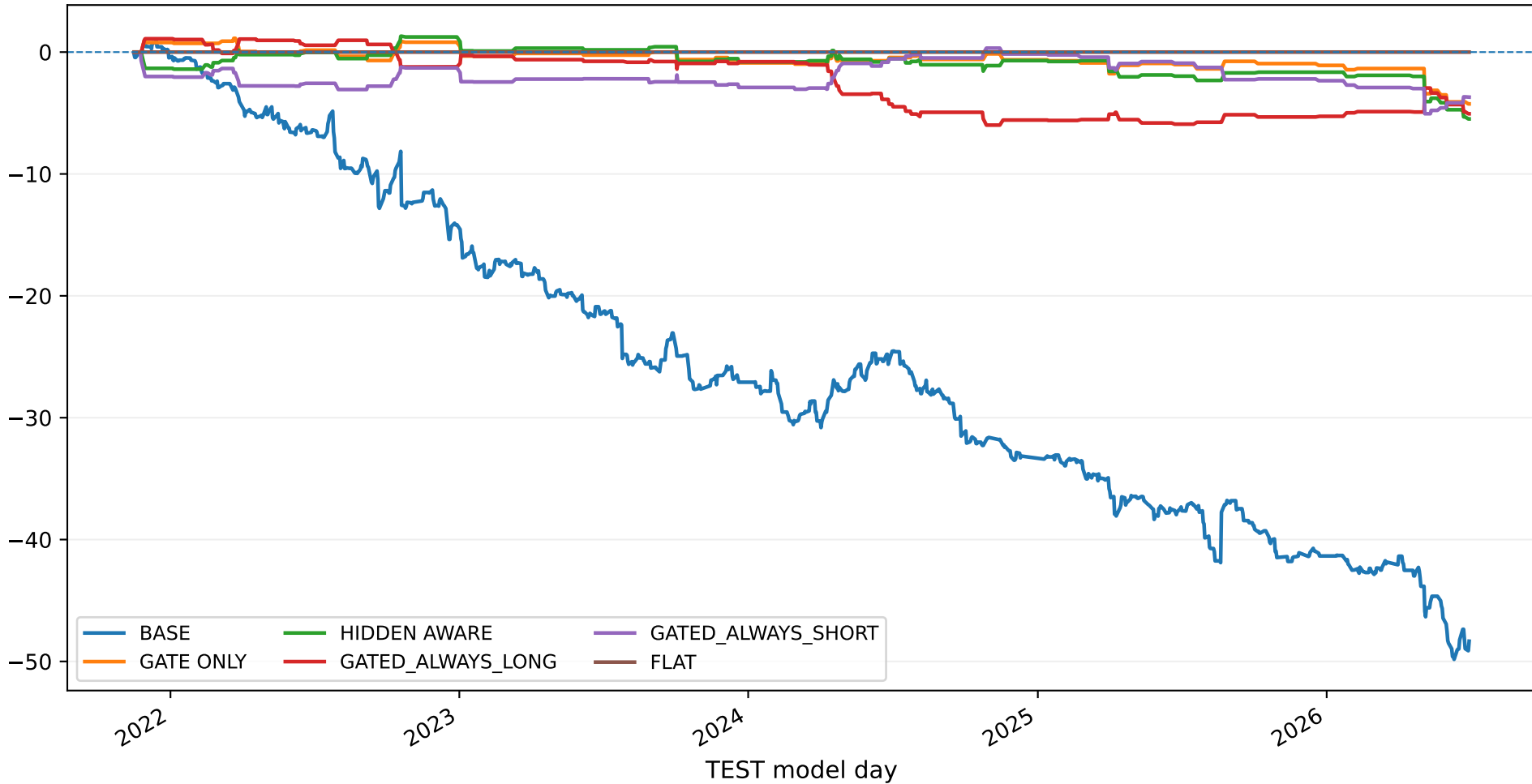
Cumulative normalised net PnL (entry-premium units)
